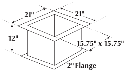
Roof Curb
